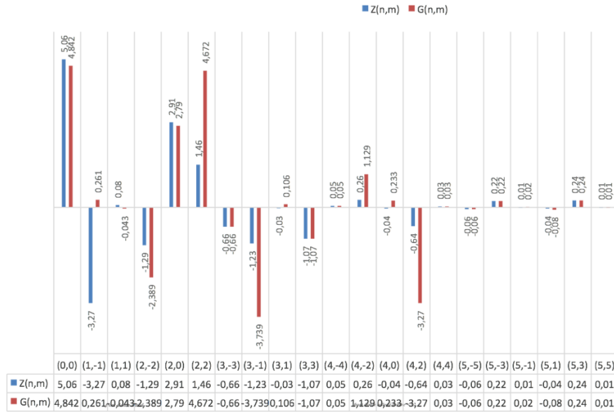
FIGURE 11. Keratoconus. Wavefront decomposition in the Zernike and the LD - HV_2 basis.
