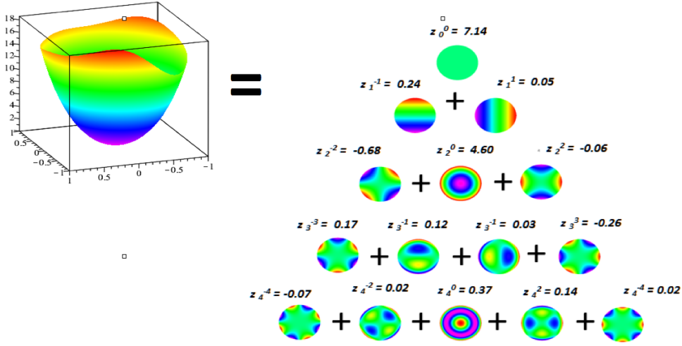
FIGURE 6. Decomposition of a quasi parabolic wavefront profile in the Zernike basis for a 5 mm pupil diameter.
