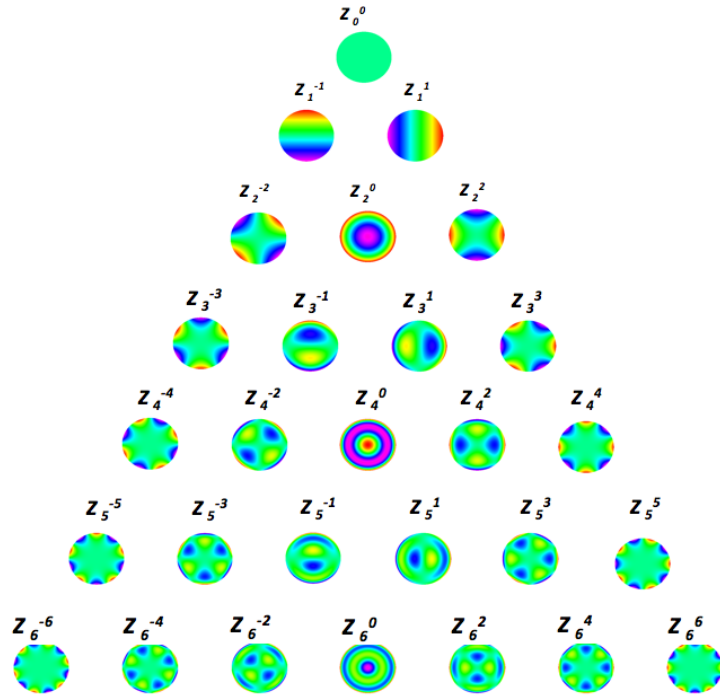
FIGURE 5. The orthonormal basis of Zernike polynomials
