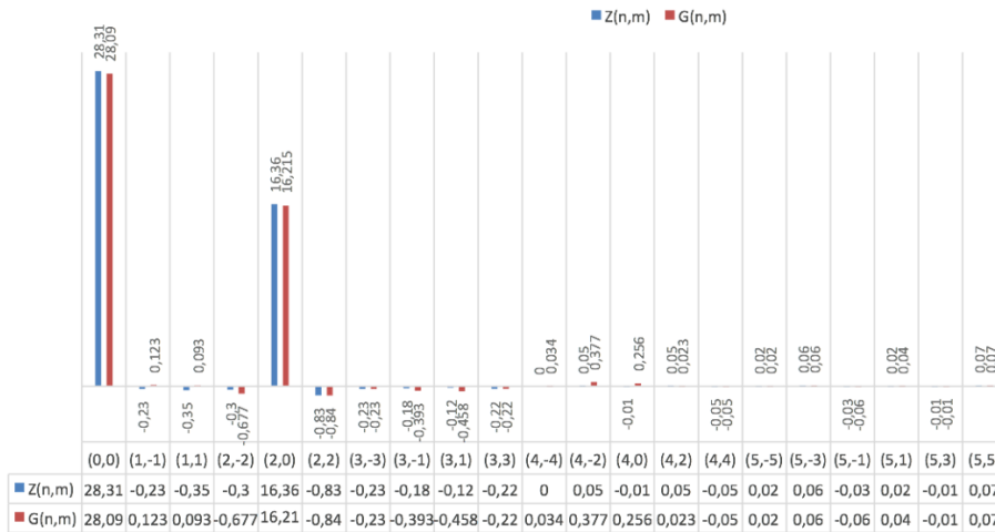
FIGURE 8. A high myopia. Wavefront decomposition in the Zernike and the LD - HV_2 basis.
