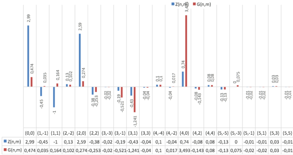
FIGURE 9. Myopia after surgery. Wavefront decomposition in the Zernike and the LD - HV_2 basis.
