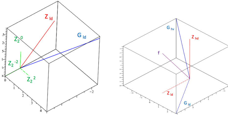
FIGURE 12. Keratoconus. The low degree contribution in Zernike and LD - HV_2 basis.
