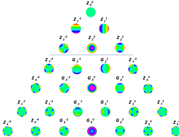
FIGURE 7. The new LD - HV_2 basis.
