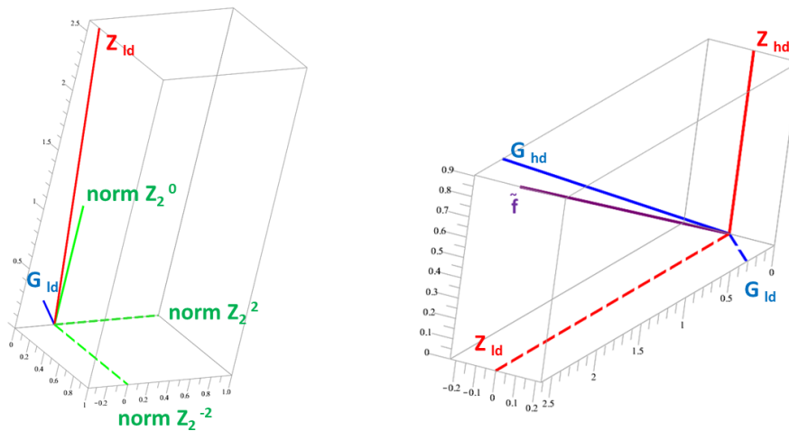
FIGURE 10. Myopia after surgery. The low degree contribution in Zernike and LD - HV_2 basis.
