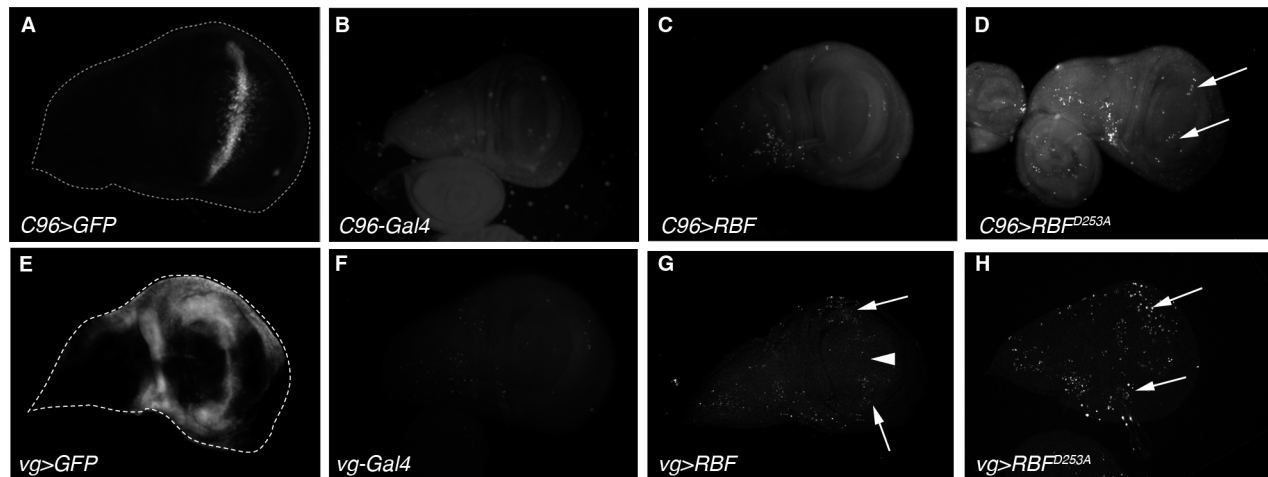
Figure 2. RBF^{D253A} is pro-apoptotic in the ZNC and induces more apoptosis than RBF in third instar larvae wing imaginal discs. (A, E) C96-Gal4 and vg-Gal4 expression patterns are visualized by UAS-mtGFP expression in third instar larvae wing imaginal discs. (B–D, F–H) Apoptotic cells are labeled by TUNEL in wing imaginal discs; specific staining of apoptotic cells corresponds to bright white patches. (B, F) C96-Gal4/+ and vg-Gal4/+ control discs have few apoptotic cells. (C) C96-Gal4/UAS-RBF wing discs are similar to control. (D) Some apoptotic cells are observed within the C96-Gal4 expression domain in UAS-RBF D253A /X; C96-Gal4/+ discs (white arrow). (G, H) Apoptotic cells are observed within the vg-Gal4 expression domain in vg-Gal4/+; UAS-RBF/+ and UAS-RBF D253A /X; vg-Gal4/+ wing discs (white arrows). (G) The white arrowhead indicates a zone at the center of the pouch where cells are not TUNEL-labeled in vg-Gal4/+; UAS-RBF/+ wing discs. All discs are shown with posterior to the top. doi:10.1371/journal.pone.0102902.g002
